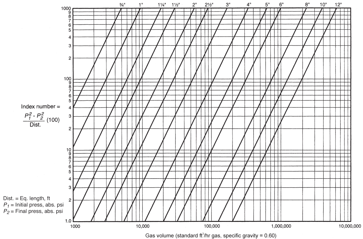
FIGURE C-A.6 (b) CAPACITY OF NATURAL GAS PIPING, HIGH PRESSURE (1.5 psi and above)
