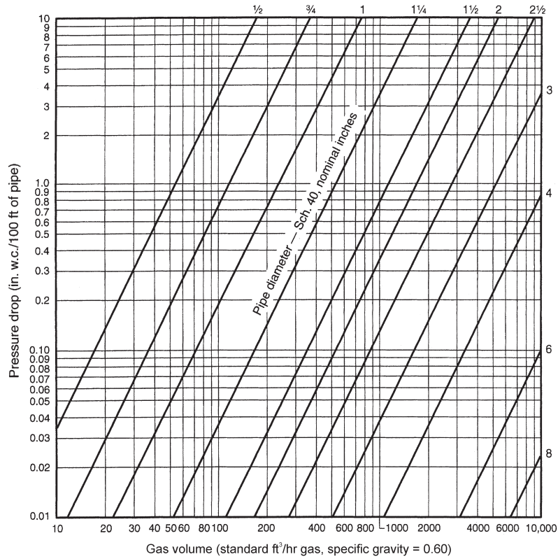
FIGURE C-A.6 (a) CAPACITY OF NATURAL GAS PIPING, LOW PRESSURE (0.60 WC)
