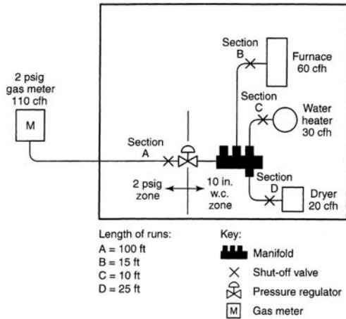
FIGURE C-A.7.2 PIPING PLAN SHOWING A CSST SYSTEM
